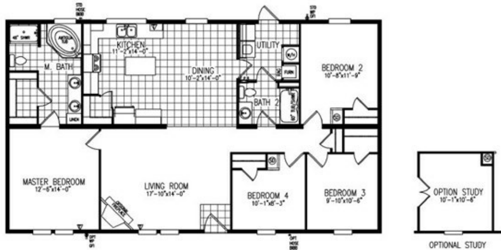
MODEL E564-230 4BR ~ 2BA 32'-0" X 56'-0" ~ 1,543 SQ. FT.
